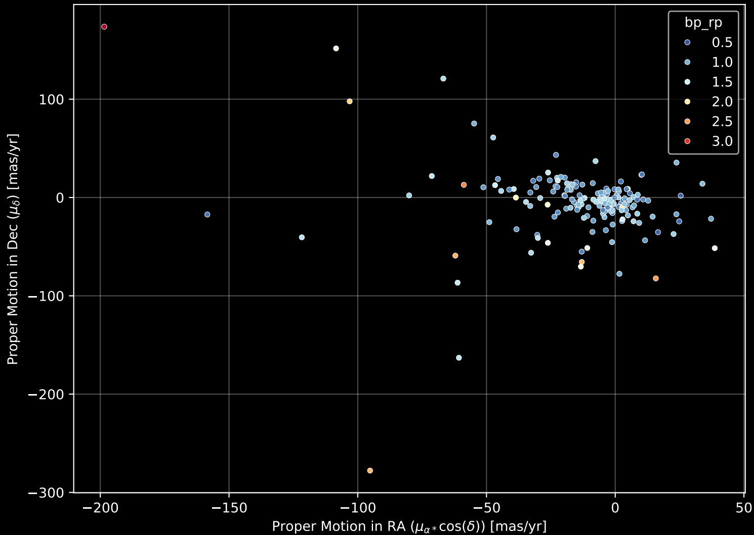
APOGEE DR17 Field: [048+55_MGA] Proper Motion Diagram (n= 172)
