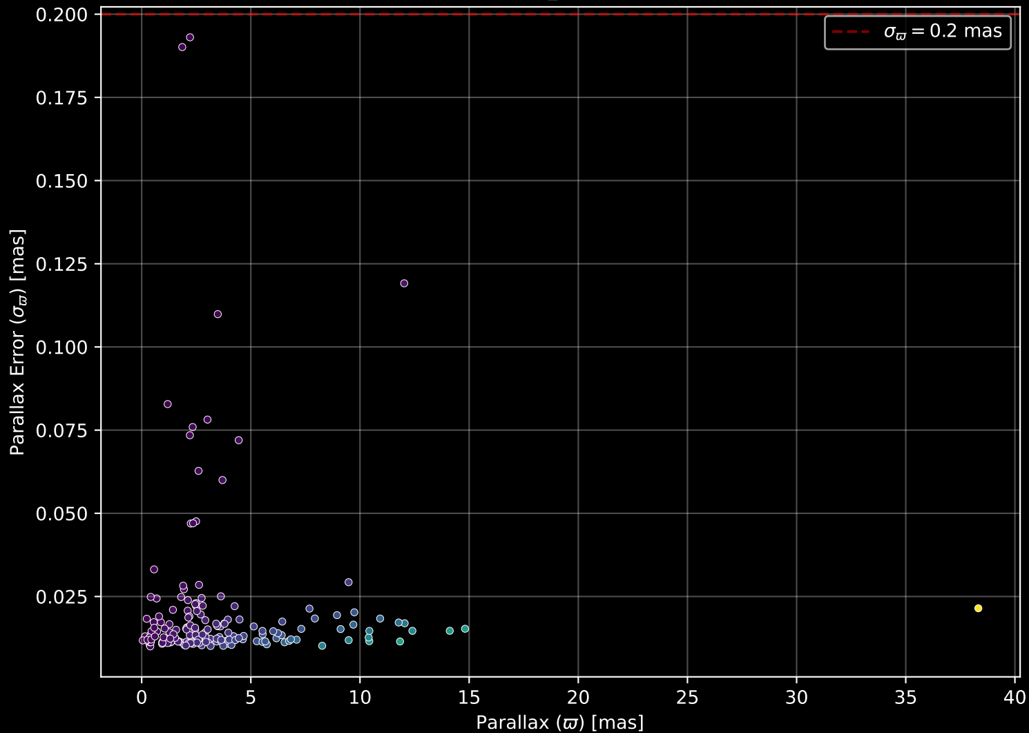
APOGEE DR17 Field: [048+55_MGA] Parallax Quality (n= 172)
