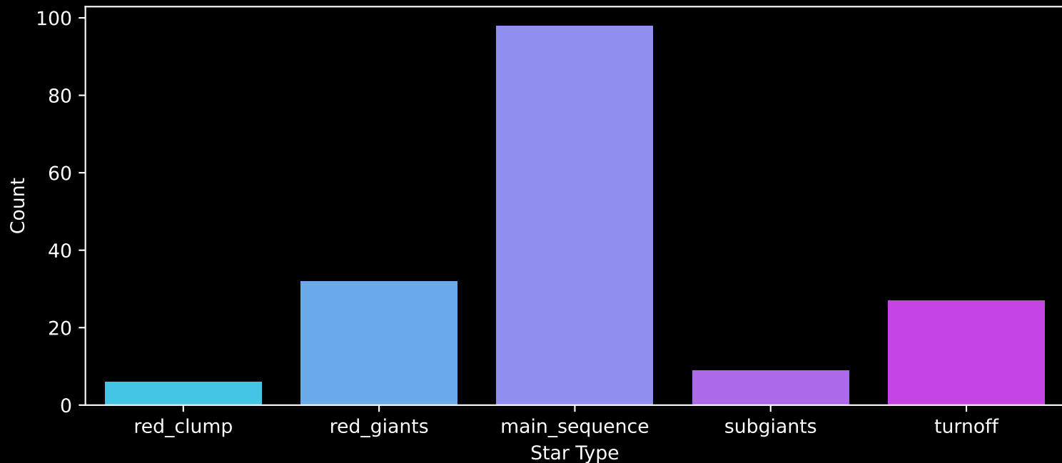
APOGEE DR17 Field: [048+55_MGA] Count plot of Star Type
