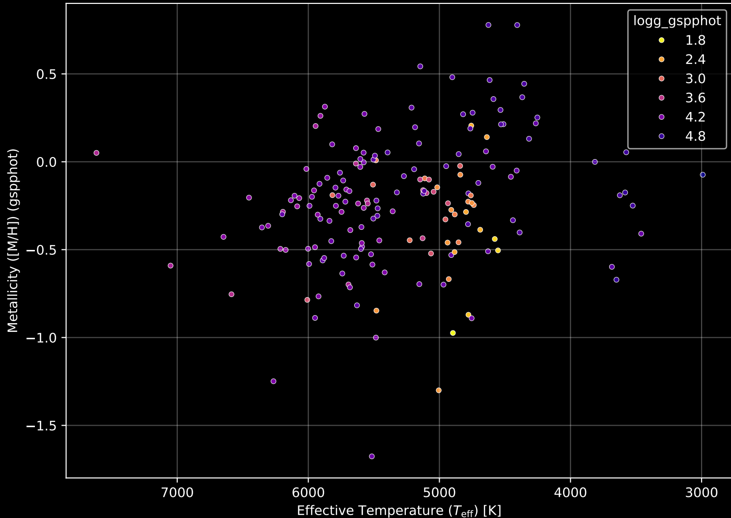
APOGEE DR17 Field: [048+55_MGA] Stellar Population Parameters (n= 172)
