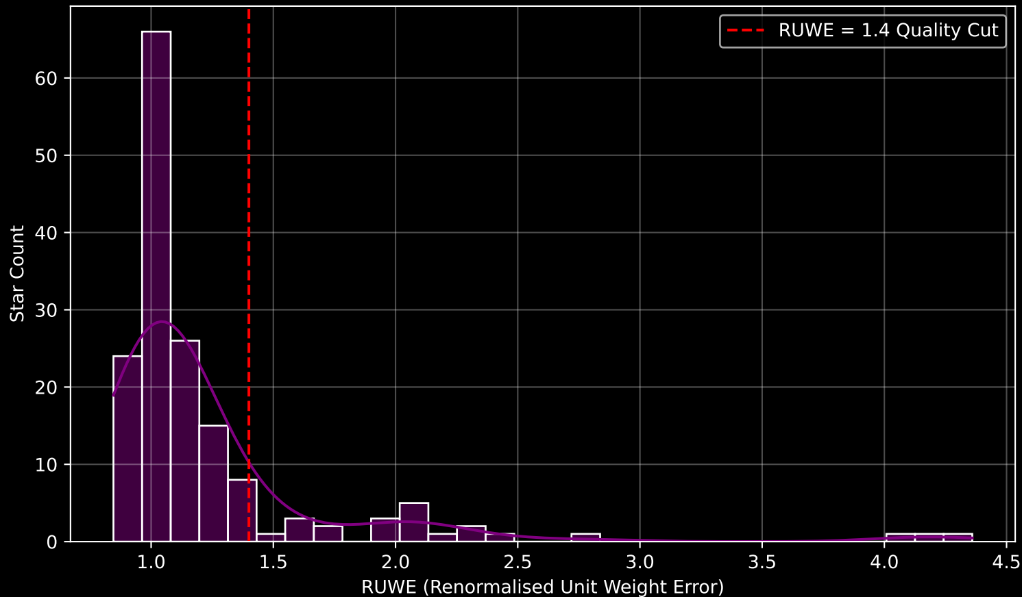
GAPOGEE DR17 Field [048+55_MGA] RUWE Distribution (n= 161)
