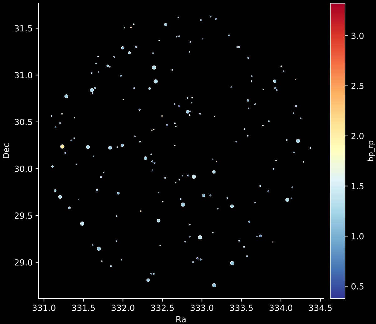
APOGEE DR17 Field: [048+55_MGA] Stars: 172
