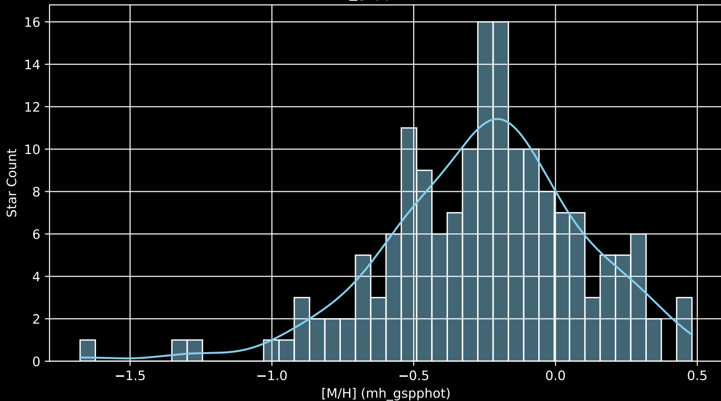
APOGEE DR17 Field: [048+55_MGA [M/H] (mh_gspphot) (n= 169)
